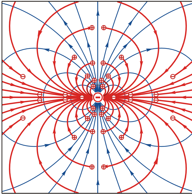
Fig. 6.2. The electromagnetic field of a magnetic dipole in a rotating frame of reference. The direction of the rotation vector is opposite to the direction of magnetic moment.
